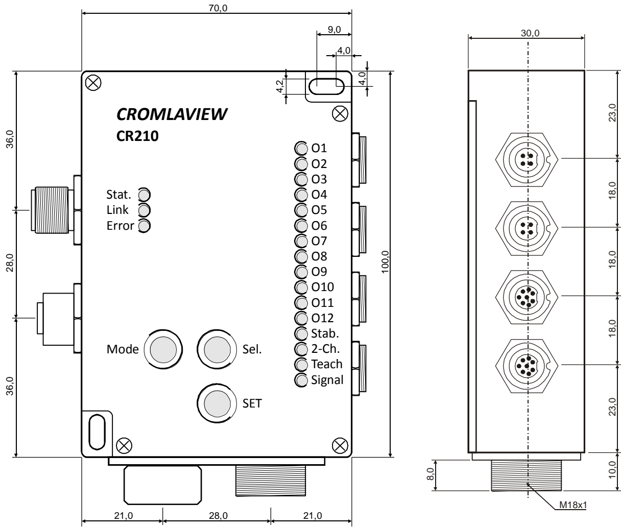
Figure 4 : Drawings CR210 with built-in control devices for the drift stabilization CROMLASTAB®
