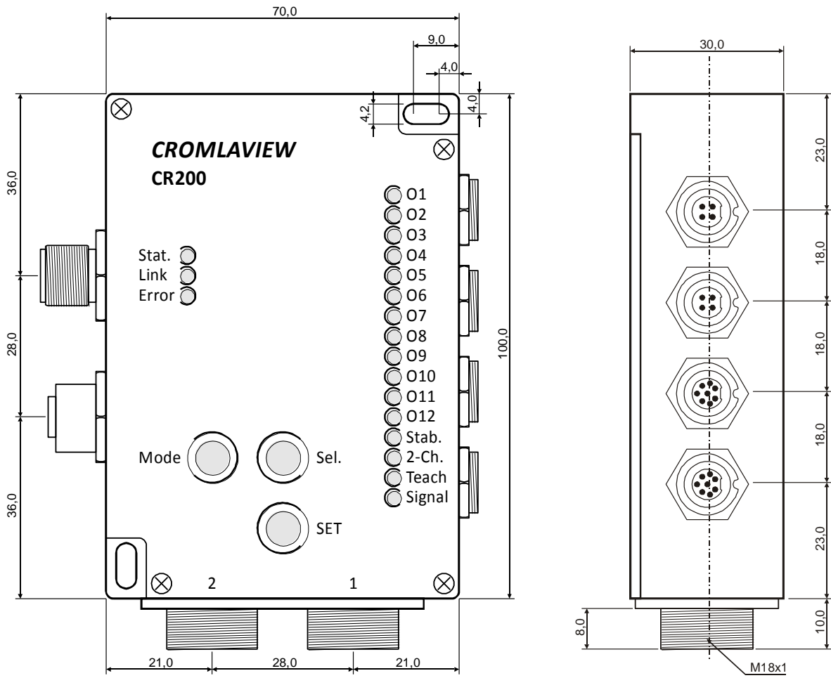
Figure 3 : Drawings CR200 for connecting two separate fiber optical cables
