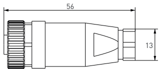
M12 Female
